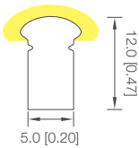
Sectional view
