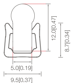
Plastic Clip ASY-NSR0512-P1NNXXX-MT
