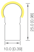
Sectional view
