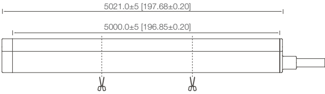
Molding pressed (IP67)
