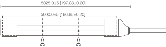
Molding pressed (IP68)
