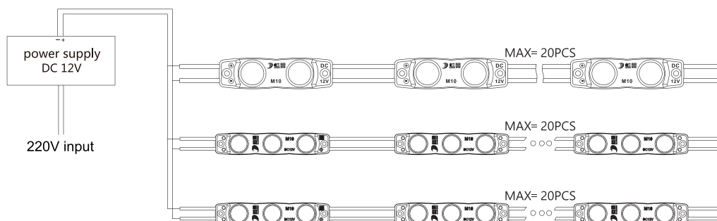
Connection Diagram
