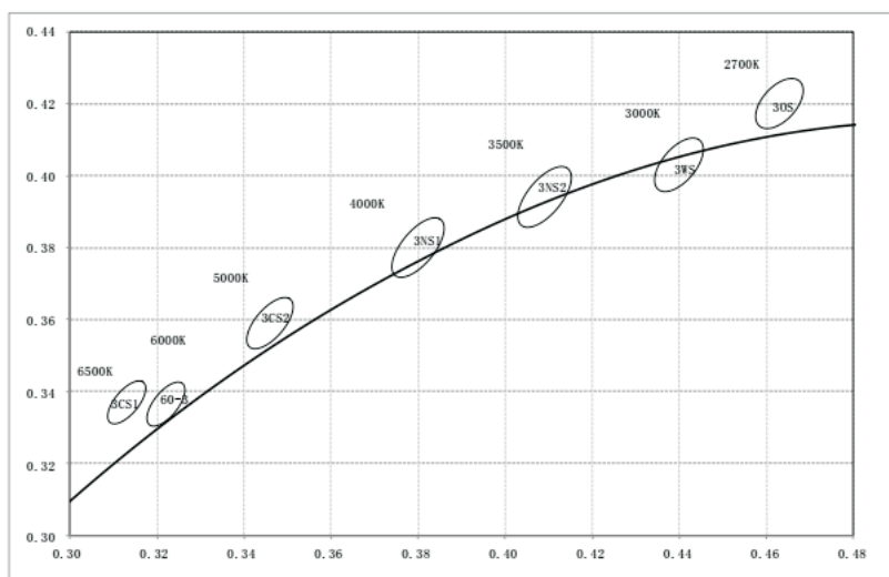
HL-AM-2835H421W-S1-08-HR3-3SDCM
