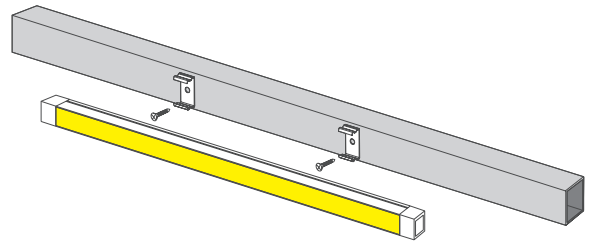
Fixed Mounting
