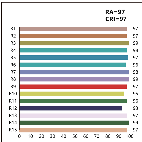
Ra chart
