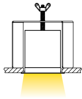
Trimmed Recessed
