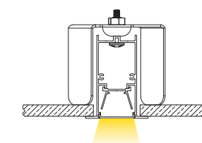
Trimmed Recessed
