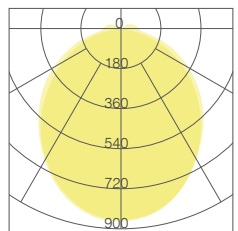
BEAM ANGLE
