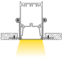
Trim-Less Recessed
