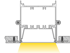
Trim-Less Recessed
