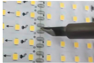
Place the soldering iron close to the position to be soldered, and the longest contact time does not exceed 3s.
