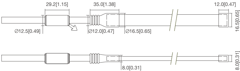
Glue Process (IP67)
