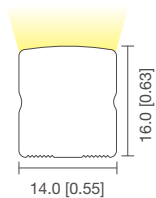
Sectional view
