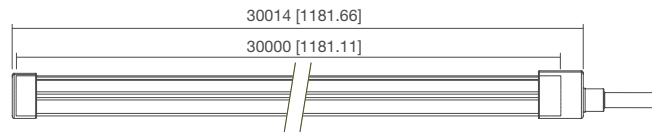
Glue Process (IP67)
